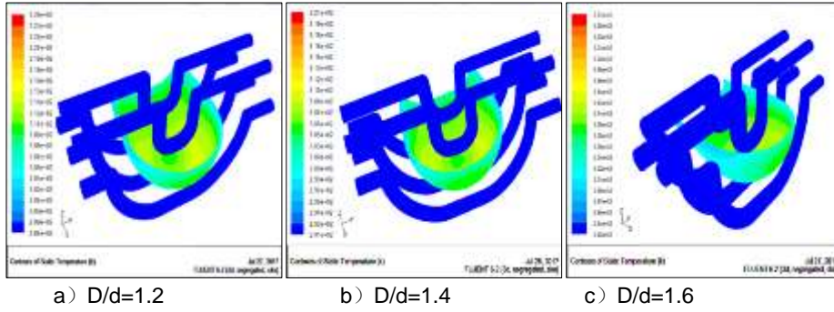
Figure 12. Temperature profile of variable cross-section cooling products.
